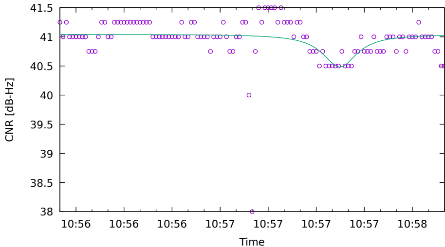
CNR fit for R02 on XiaomiMi8 - drive 10 (DOY263)
