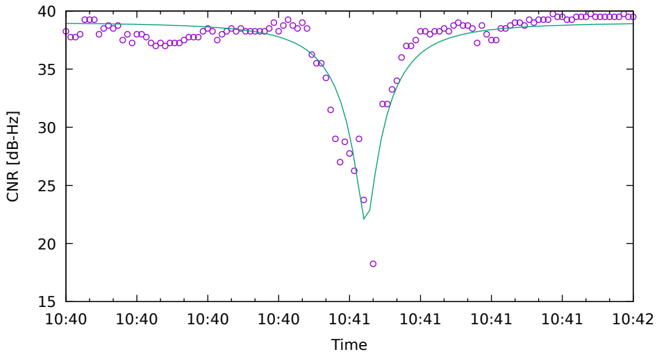
CNR fit for R17 on XiaomiMi8 - drive 1 (DOY263)
