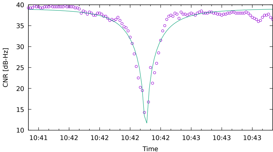
CNR fit for R17 on XiaomiMi8 - drive 2 (DOY263)
