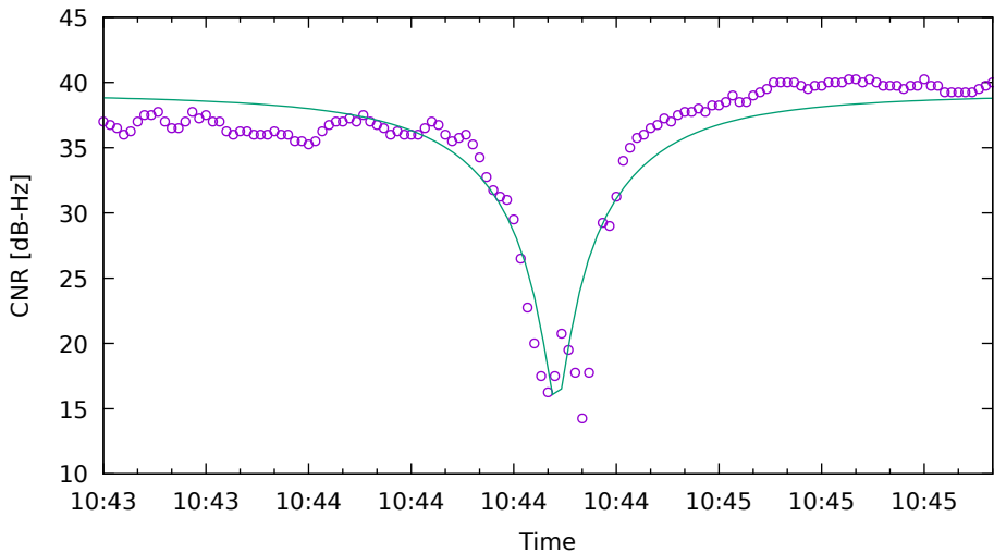
CNR fit for R17 on XiaomiMi8 - drive 3 (DOY263)
