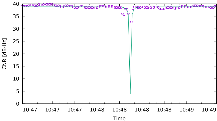
CNR fit for R17 on XiaomiMi8 - drive 5 (DOY263)
