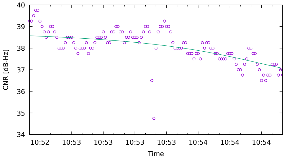
CNR fit for R17 on XiaomiMi8 - drive 8 (DOY263)
