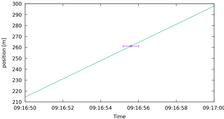
Jamer position fit DOY262 S1 D1
