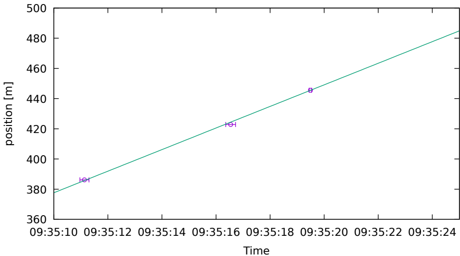
Jammer position fit DOY262 S1 drive 10
