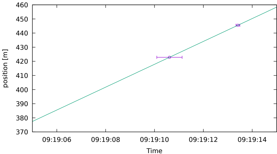
Jammer position fit DOY262 S1 drive 2
