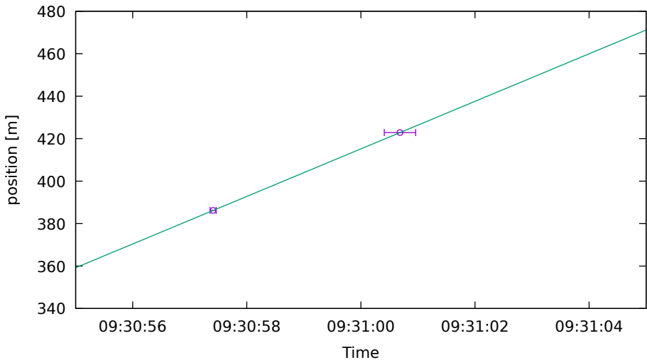
Jammer position fit DOY262 S1 drive 8
