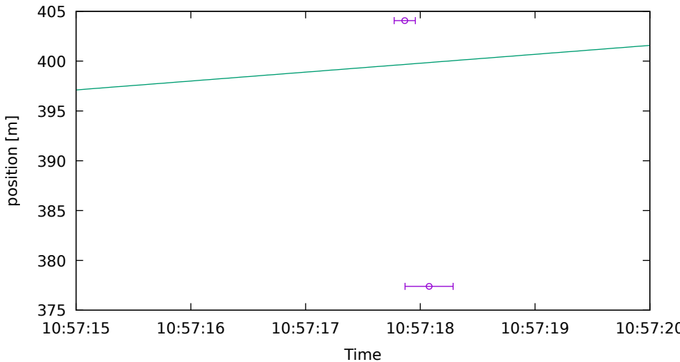
Jammer position fit DOY262 S2 drive 8
