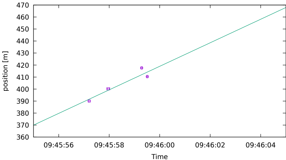
Jammer position fit DOY263 S2 drive 4
