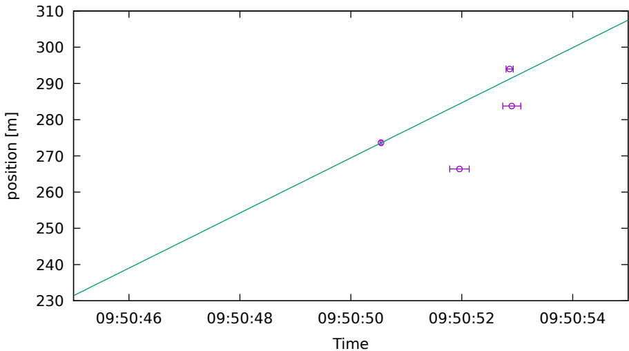
Jammer position fit DOY263 S2 drive 7
